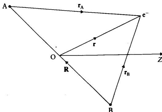
13.9 A coordinate system for the discussion of an H^+ + H collision. Note that the position vector r of the electron can be in any direction whereas the vector R lies in the plane of motion of A and B, which has been taken to be the XZ plane (see Fig. 13.8).
